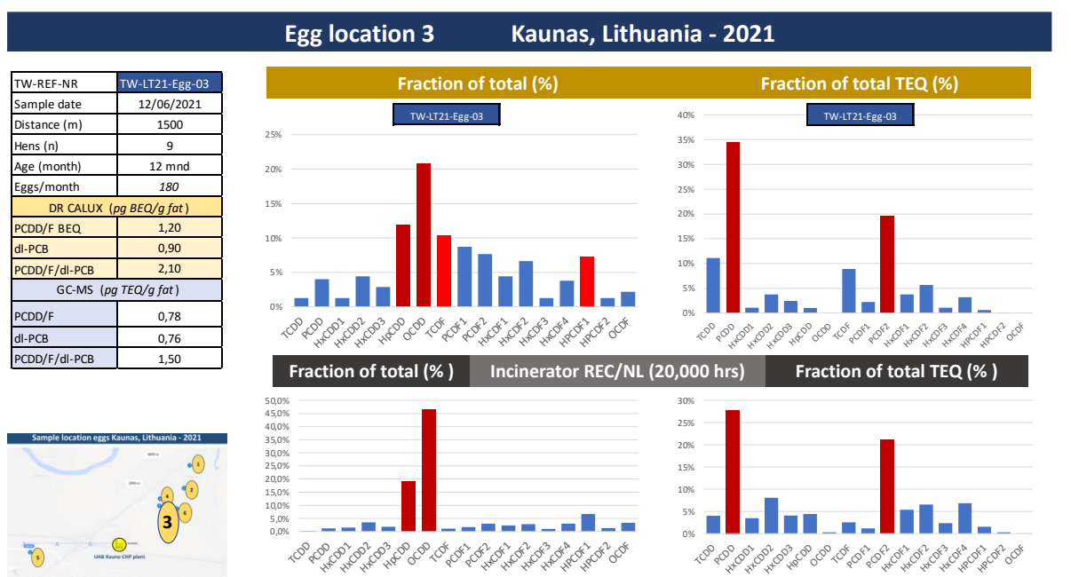
Figure 25: Results of dioxin analysis of egg location 3, Kaunas – 2021
