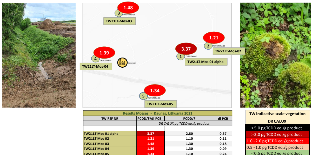
Figure 38: Sum of dioxins (PCDD/F/dl-PCBs) in mosses – Kaunas 2021
