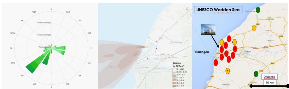
Figure 3: Wind rose for Harlingen, NL, with dominant average wind direction from SW (a), dioxin cloud during calamity, 2015 (b), contaminated backyard chicken eggs, Harlingen (c)
