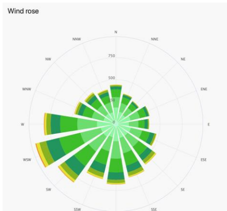
Figure 2: Annual and 2-week wind rose for Kaunas, Lithuania
