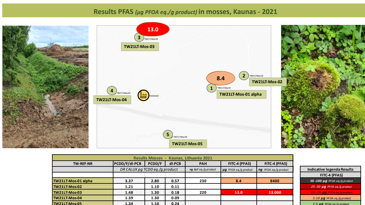
Figure 44: PFAS in mosses – Kaunas 2021
