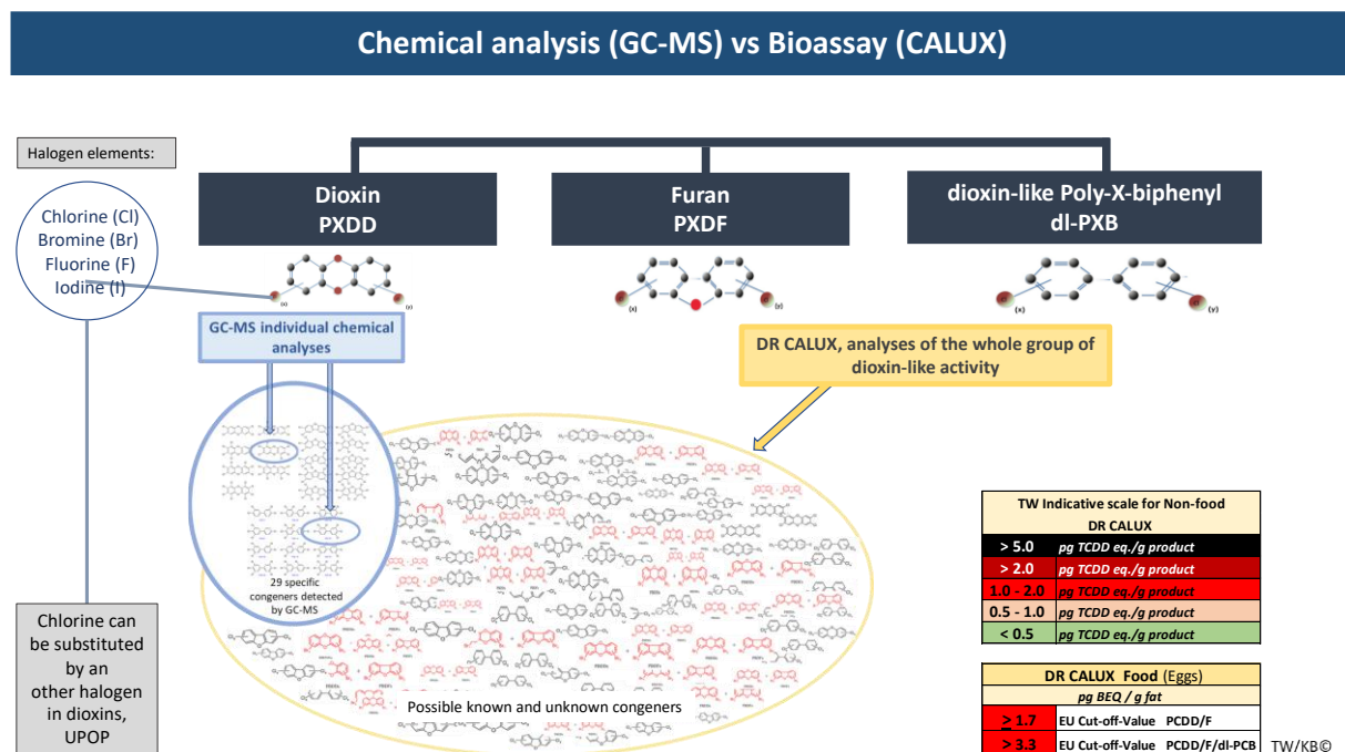
Figure 5: Chemical GC-MS analysis vs bioassay DR CALUX analysis, ©ToxicoWatch
