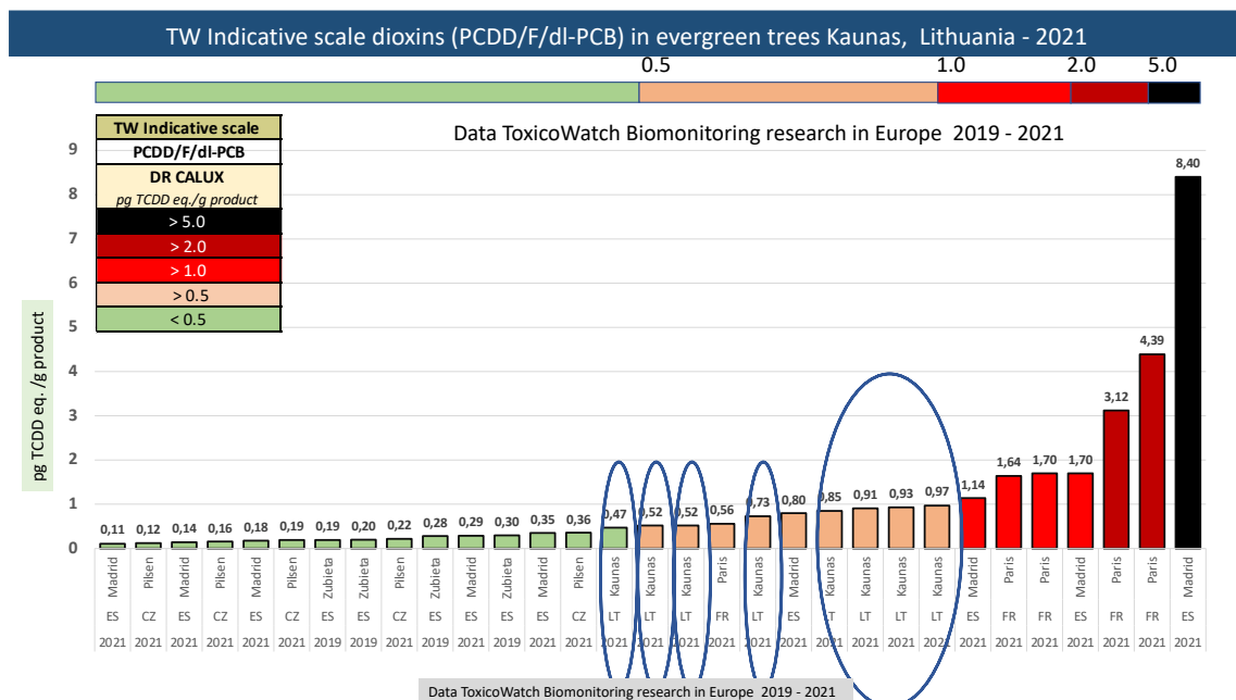
Figure 34: Indicative scale – dioxins (PCDD/F/dl-PCB) in pine needles in Europe using DR CALUX
