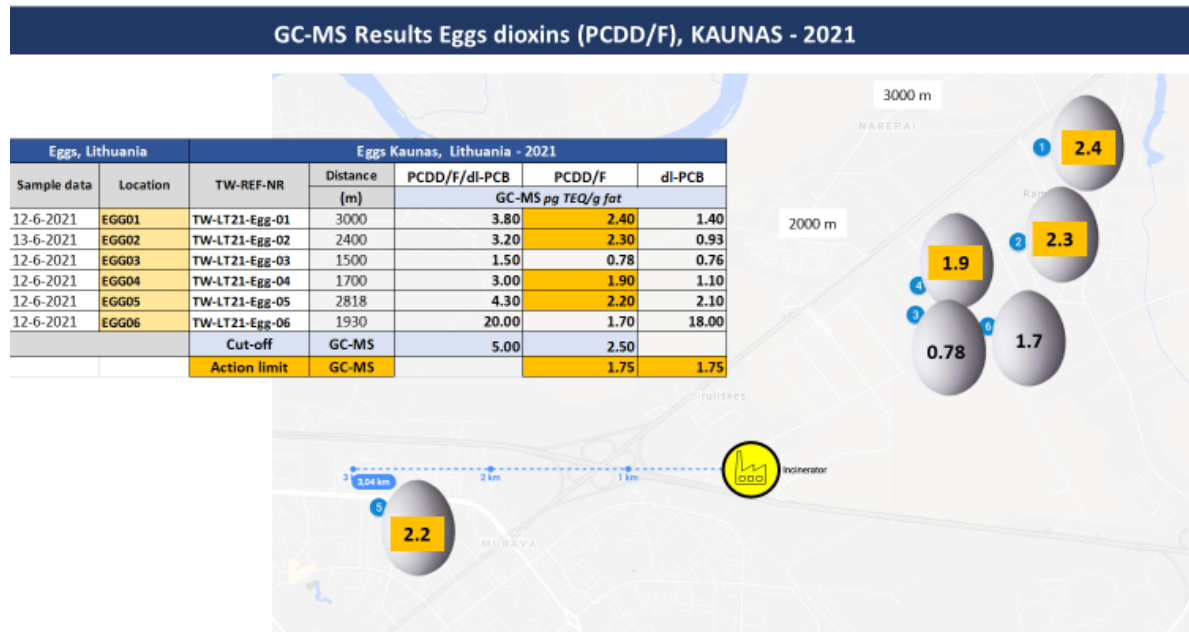
Figure 20: Exceeding EU action limit for dioxins (PCDD/F) in eggs by GC-MS analysis – Kaunas 2021
