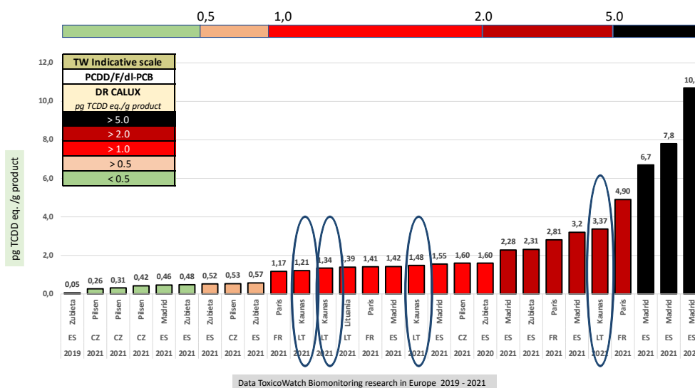
Figure 39 TW indicative scale overview of dioxins (PCDD/F/dl-PCB) in mosses of Europe (TW research)
