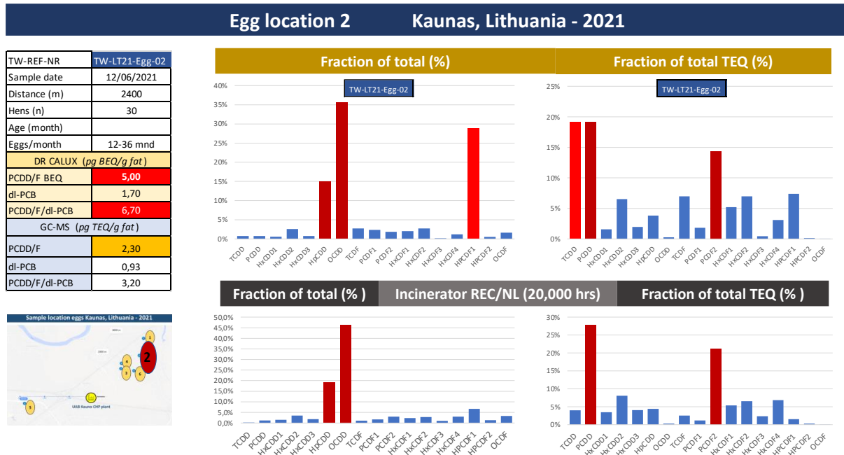
Figure 24: Overview of data, egg location 2 Kaunas – 2021, see Annex II Eggs
