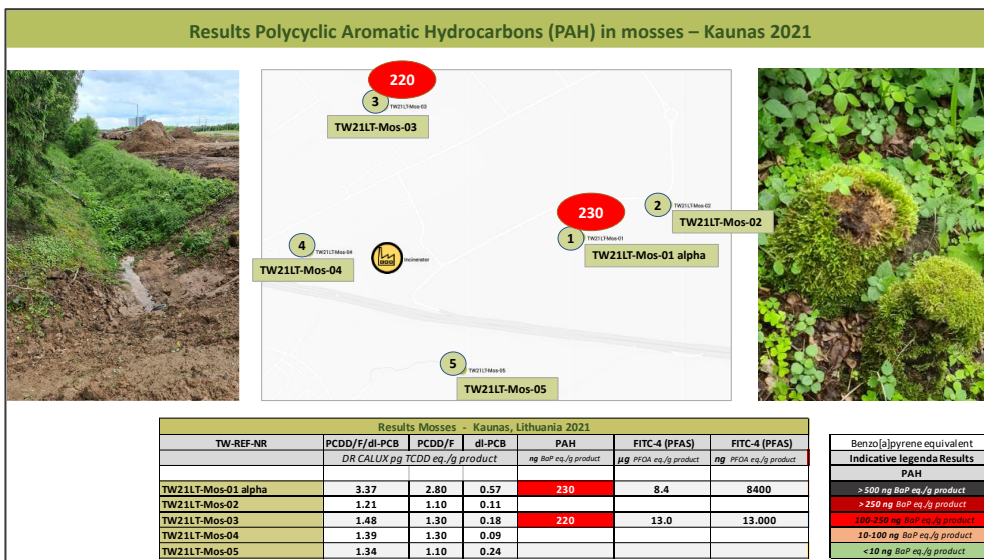
Figure 42: Polycyclic Aromatic Hydrocarbons (PAHs) in mosses – Kaunas 2021
