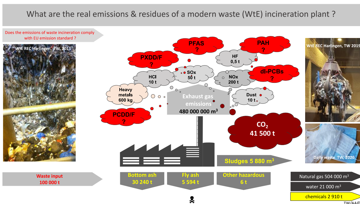
Figure 7: What are the real emissions of WtE incineration? © TW
