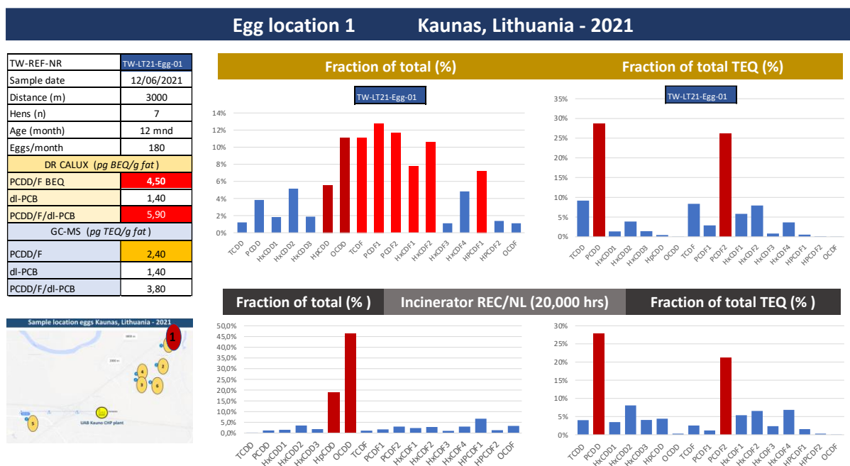
Figure 23: Overview of data, egg location 1 Kaunas – 2021, see Annex II Eggs
