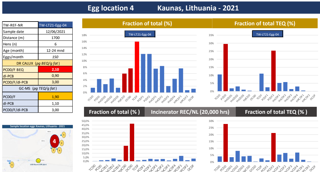
Figure 26: Results of dioxin analysis of egg location 4, Kaunas – 2021
