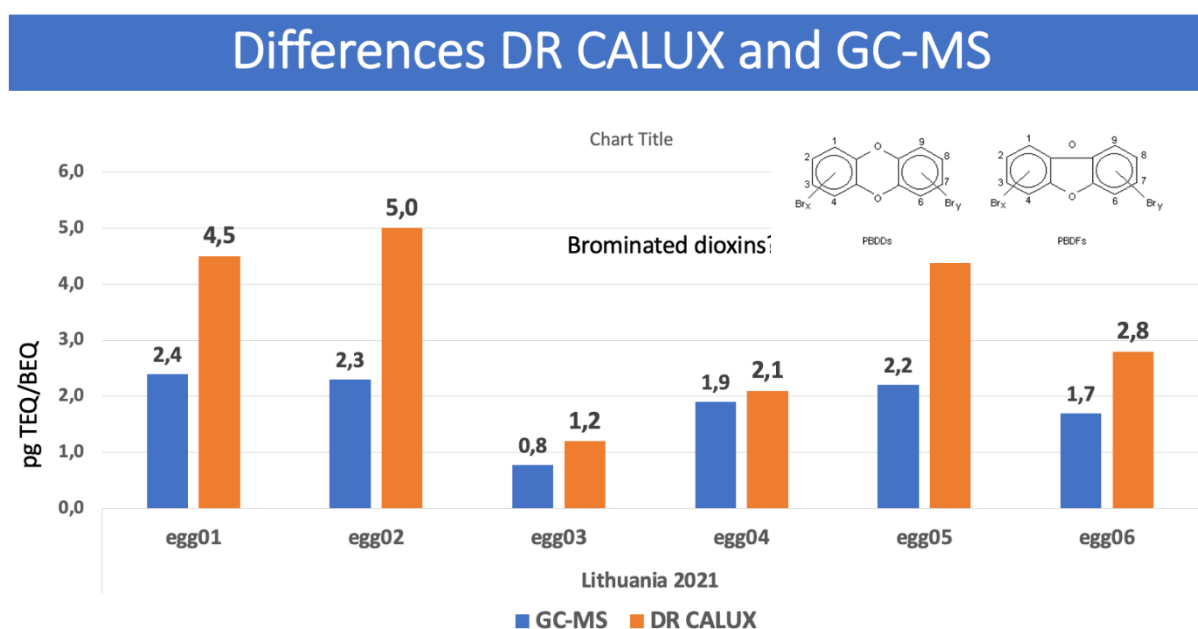
Figure 30: Difference between GC-MS and DR CALUX indicates evidence of brominated dioxins
