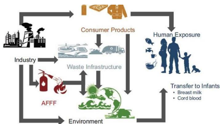
Figure 11: PFAS exposure pathways to the human population and the environment (Sunderland et al. 2019)
